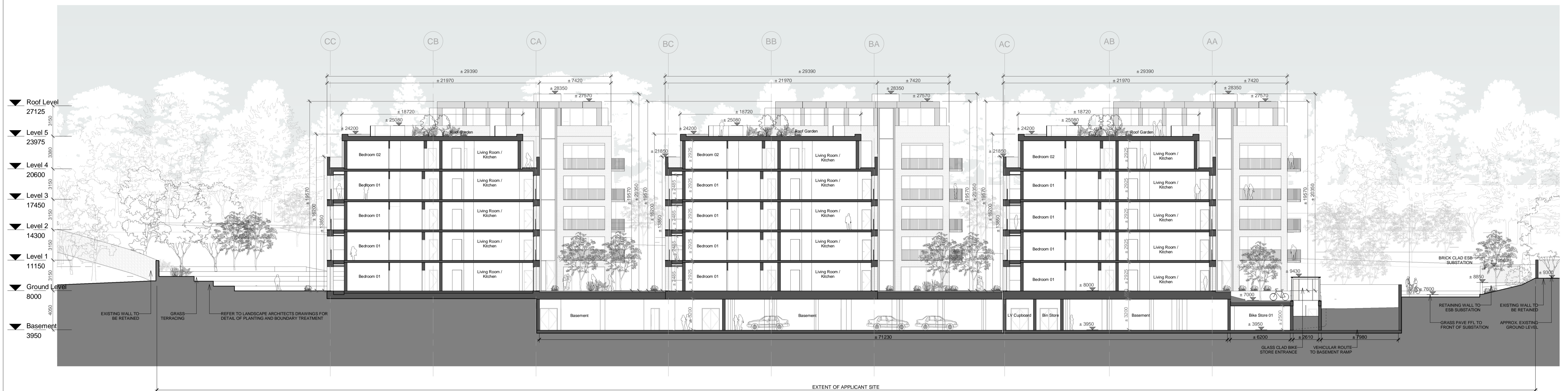
1 Building Section AA scale 1 : 200
