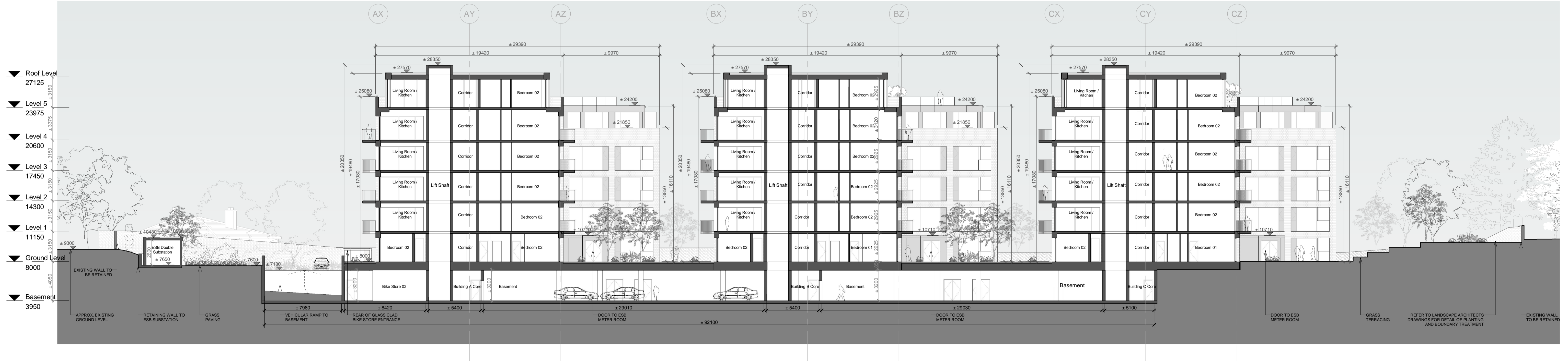
2 Building Section BB scale 1 : 200
